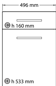
Cassetto + anta Drawer + door / Tiroir + porte / Schublade + Tür Cajon + puerta
